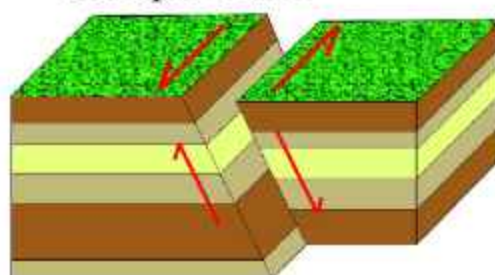
Fig. 2.11: Types of Faults
