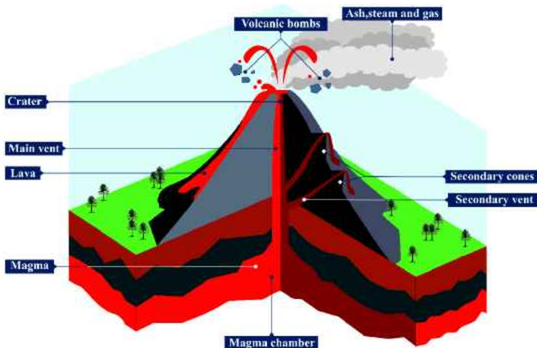
Fig. 2.13: Volcanoes
