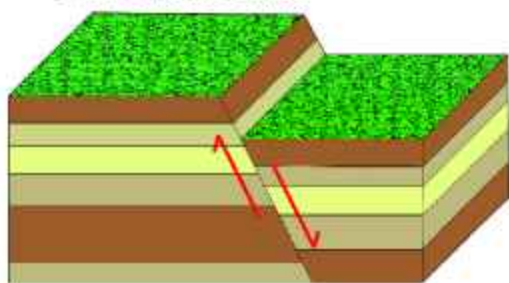
Normal Fault
