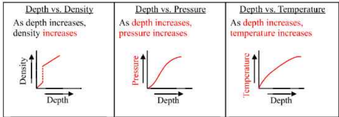
Fig. 2.1: Density, Pressure and Temperature with Depths
